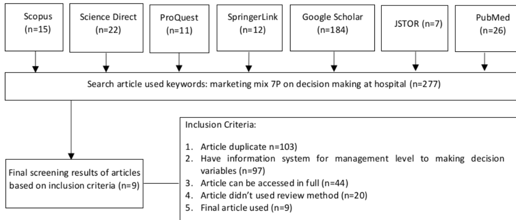
Figure. Flow Chart Screening Article
