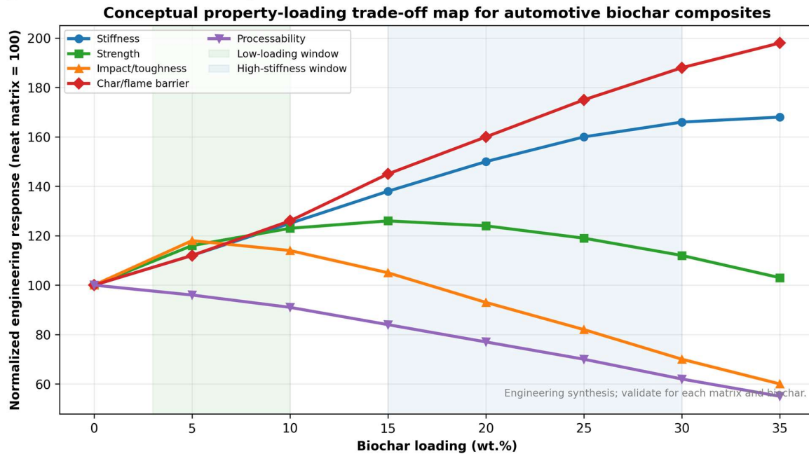
Figure 2. Conceptual Property-Loading Trade-Off Map for Biochar Composites. The Curves Synthesize Trends Reported Across Different Polymer Matrices and Are Intended as Engineering Design Guidance
